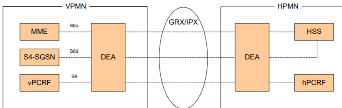
Figure 3 - GSMA roaming implementation architecture
