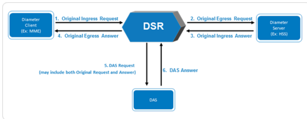
Figure 71 - Message Copy Overview
