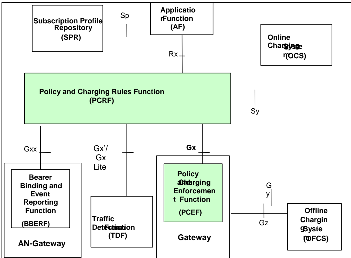
Figure 59 - Overall PCC logical architecture (non-roaming)
