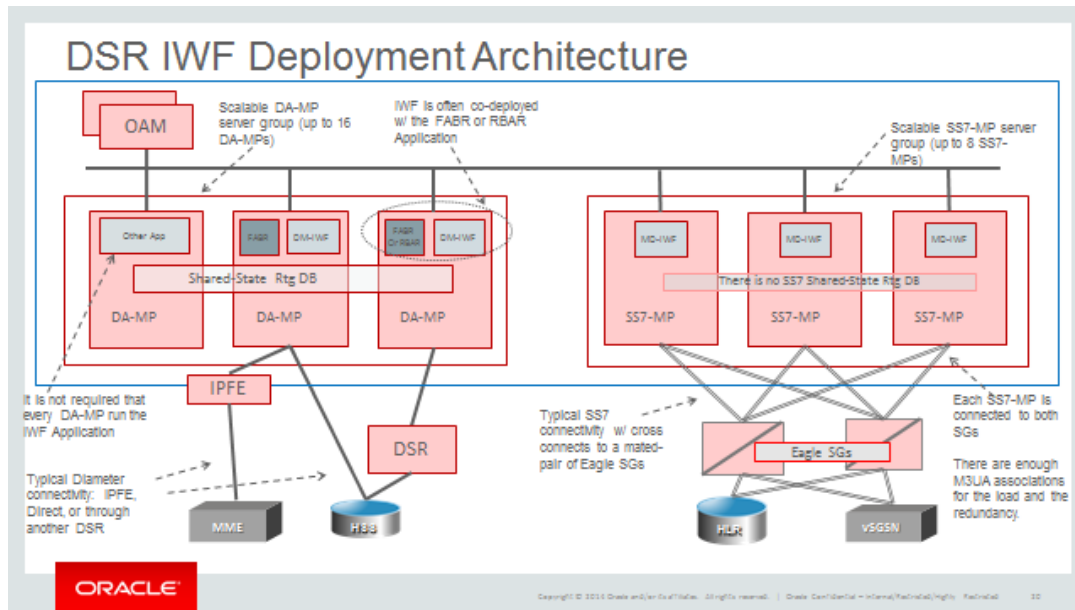
Figure 55 - DSR with MAP-Diameter IWF
