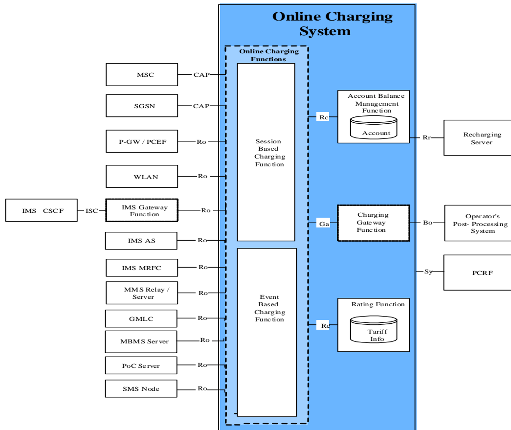
Figure 56 - Online Charging System and Architecture
