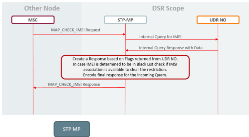
Figure 80 – SS7 EIR call flow
