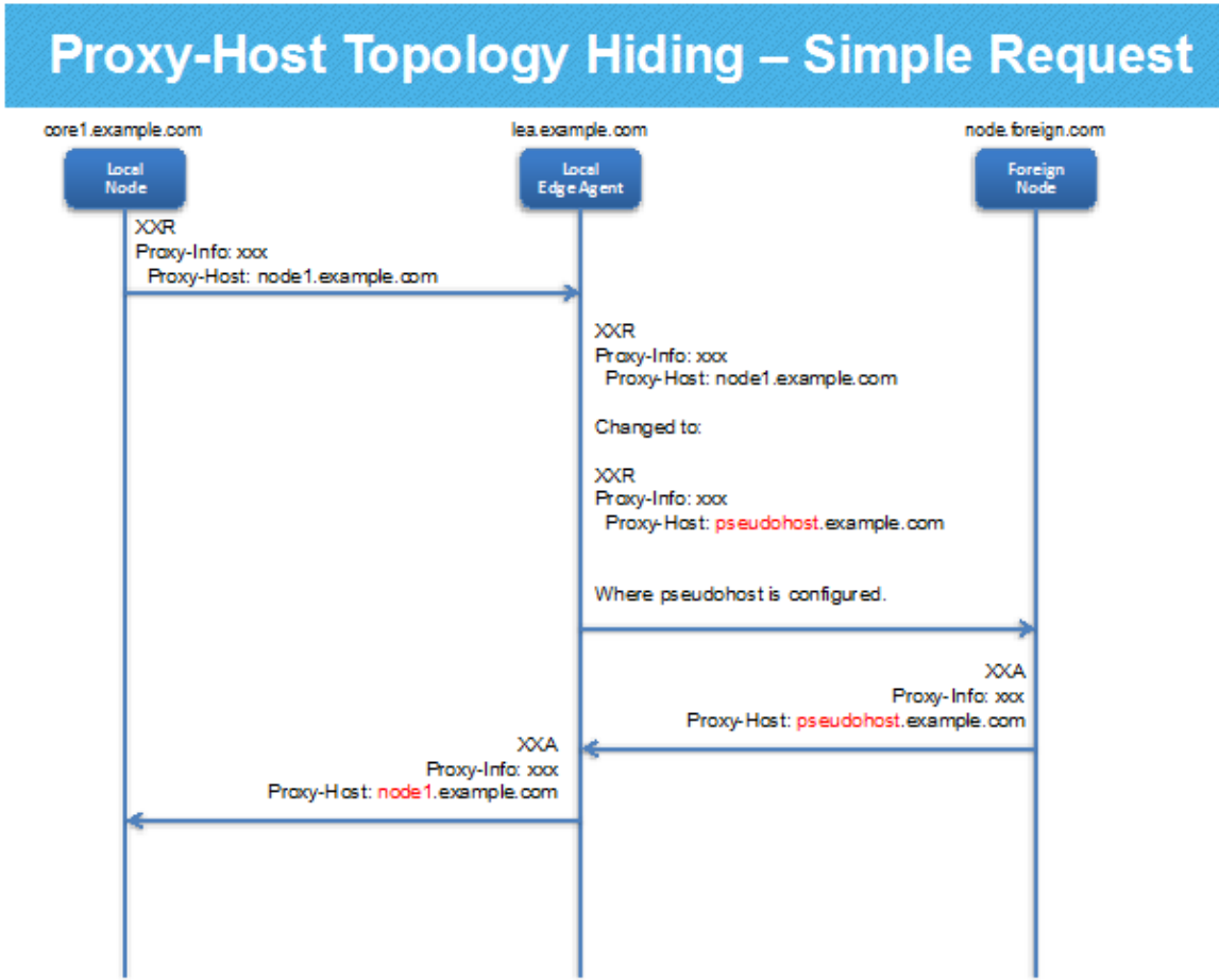
Figure 52 - Proxy-Host Topology Hiding Message Flow
