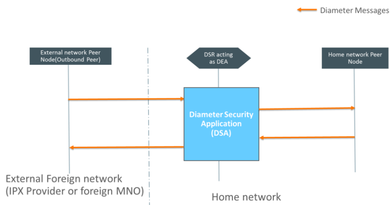
Figure 67 – Diameter Security Application (DSA)
