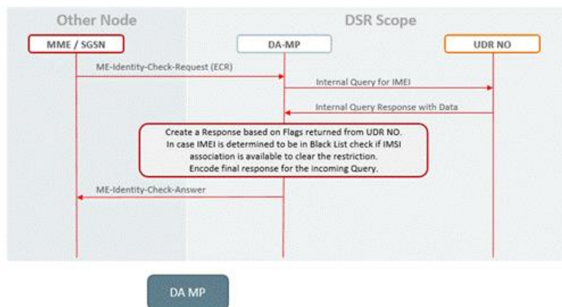
Figure 81 – S13 EIR Call Flow
