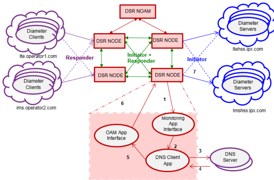
Figure 17 – Dynamic Diameter Peer Discovery: Example
