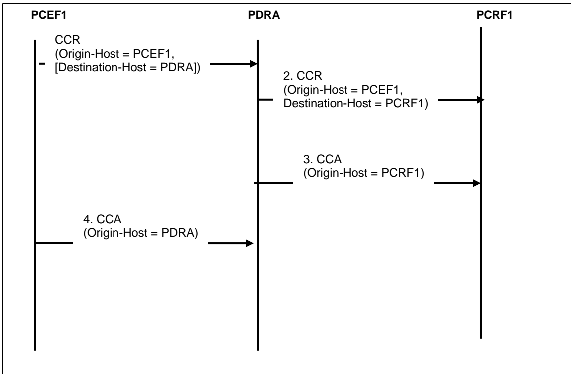
Figure 60 - PCRF topology hiding
