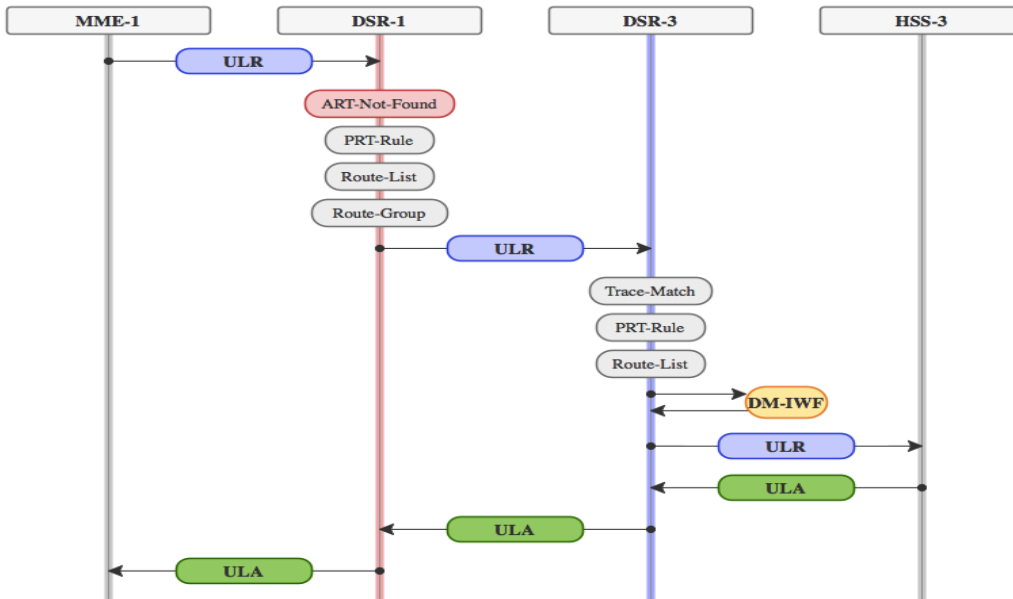
Figure 77 – Message Flow for Network Wide Trace
