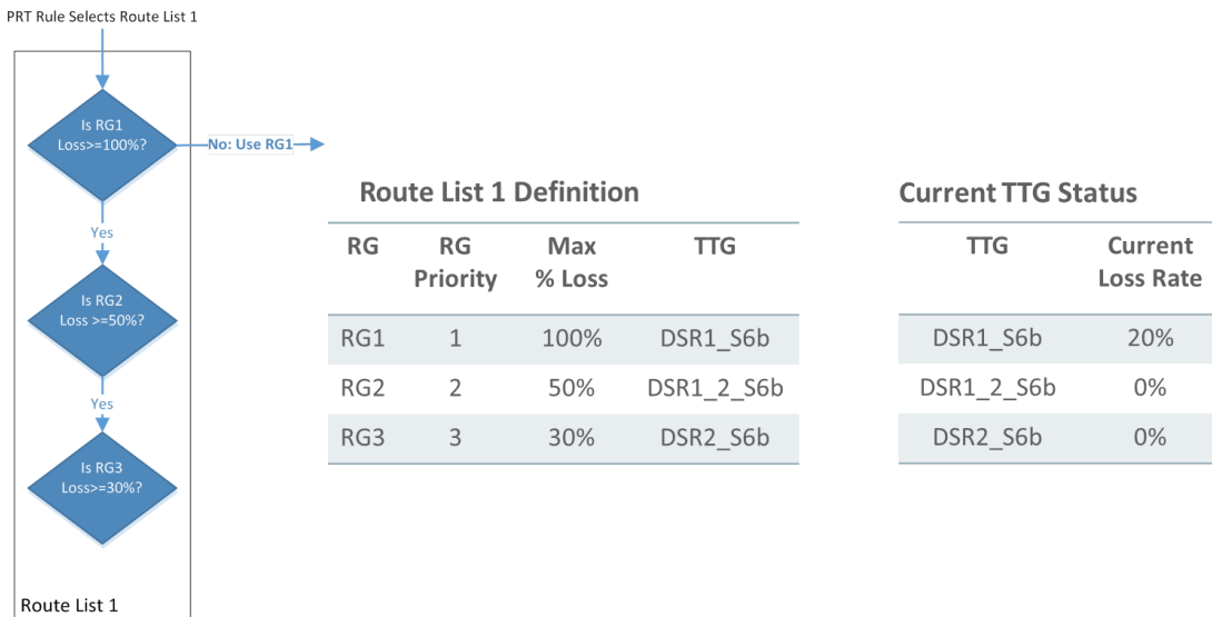
Figure 37 - Congestion-Aware Route List Logic
