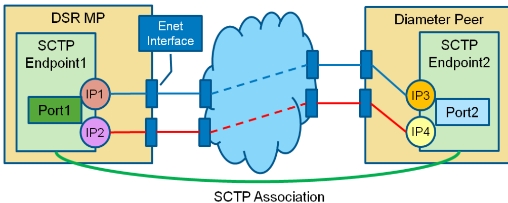
Figure 15 - SCTP Multi-Homing
