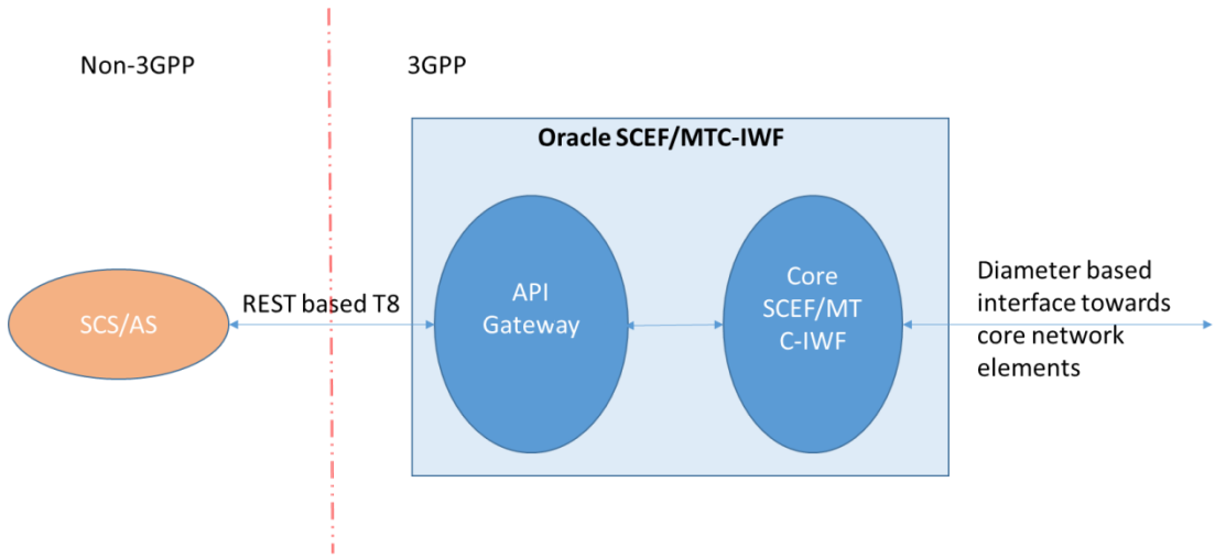
Figure 68: Functional view of SCEF/MTC-IWF functionality at DSR
