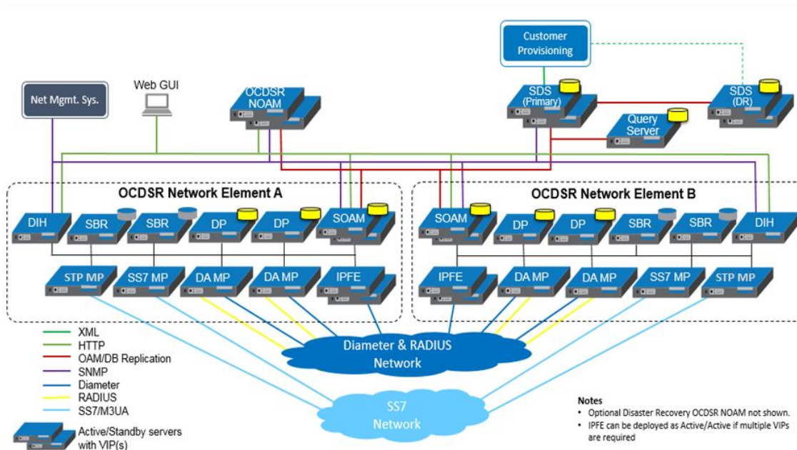
Figure 5 - DSR 7.x Architecture
