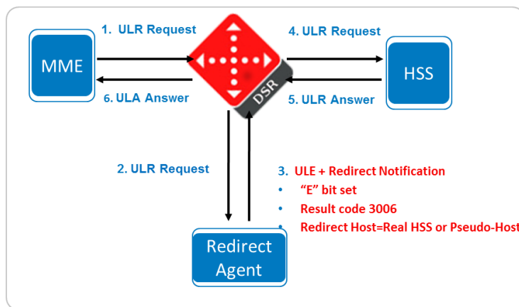
Figure 14 - Redirect Agent
