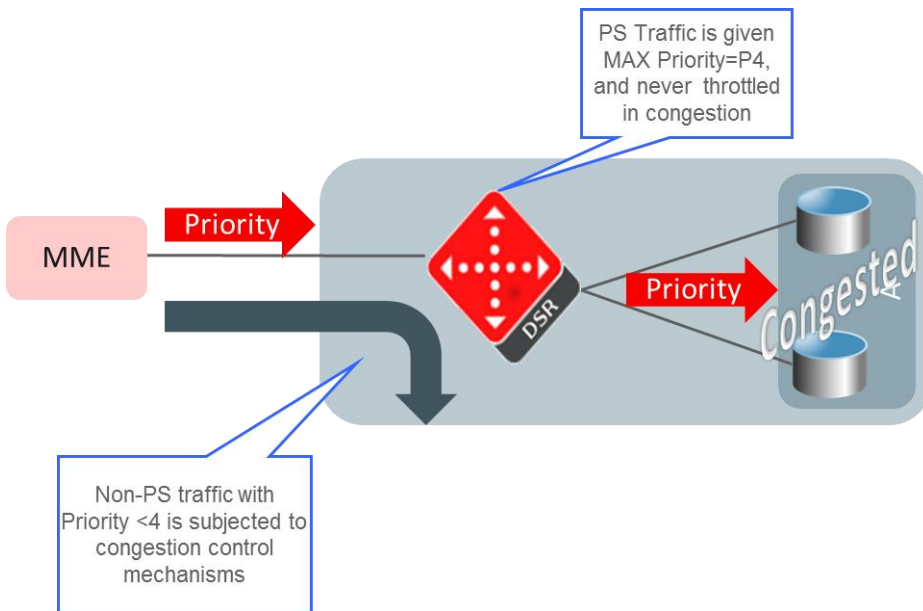
Figure 41 - NGN-PS Support
