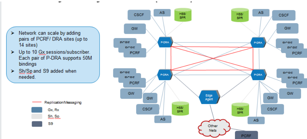
Figure 63 - PCA Example Deployment
