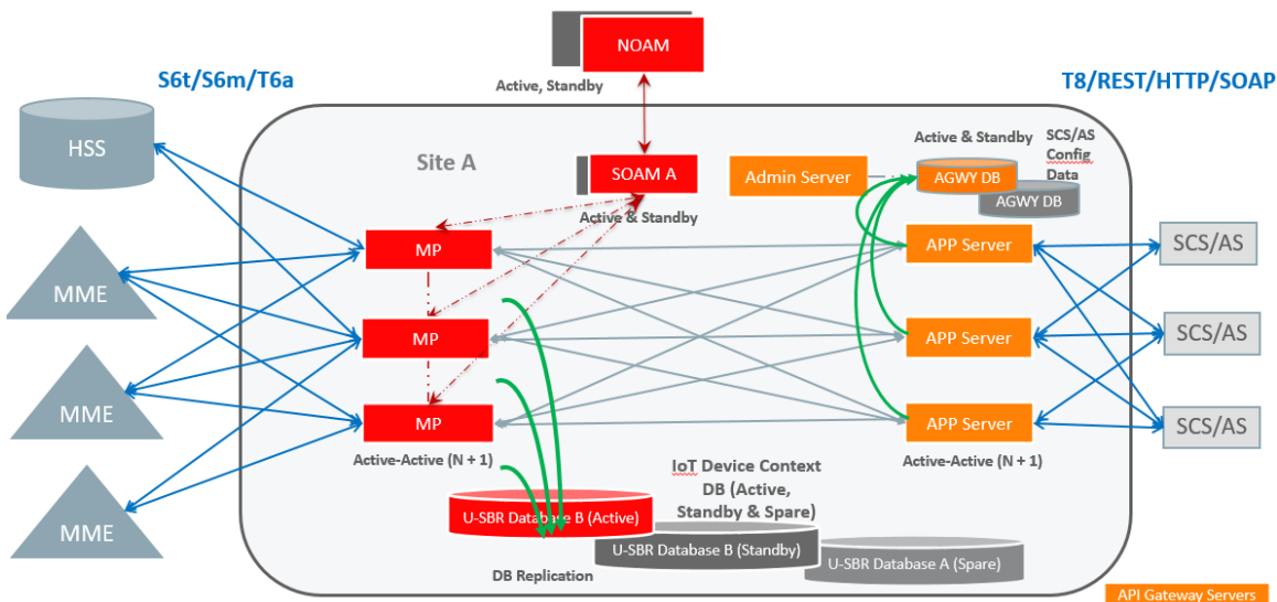
Figure 69: SCEF site architecture example
