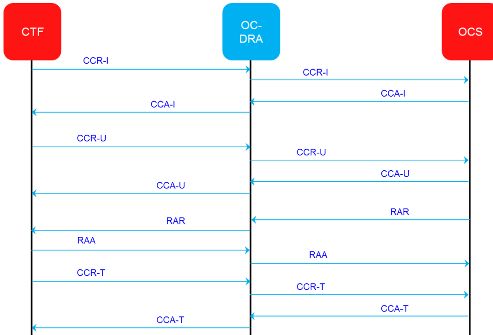
Figure 57 - A typical Online Charging Session
