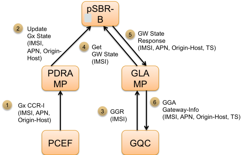
Figure 64 - IMSI Query with Single Matching Gx Session Use Case
