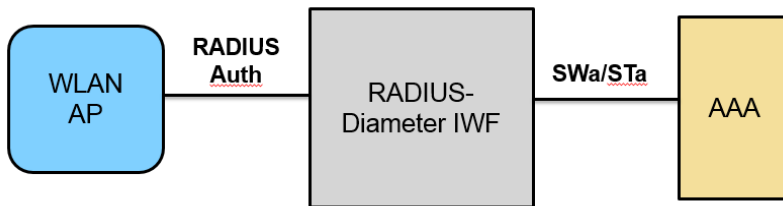
Figure 45 - RADIUS-Diameter IWF for WLAN Authentication
