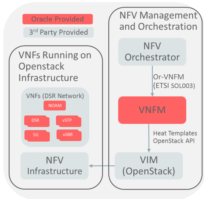
Figure 72 – DSR VNFM
