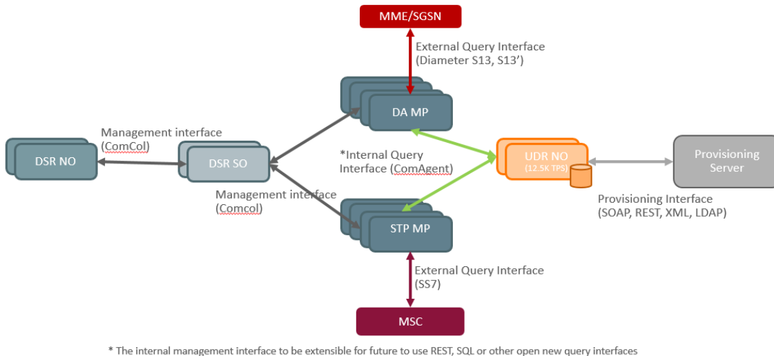
Figure 79 – EIR solution architecture.
