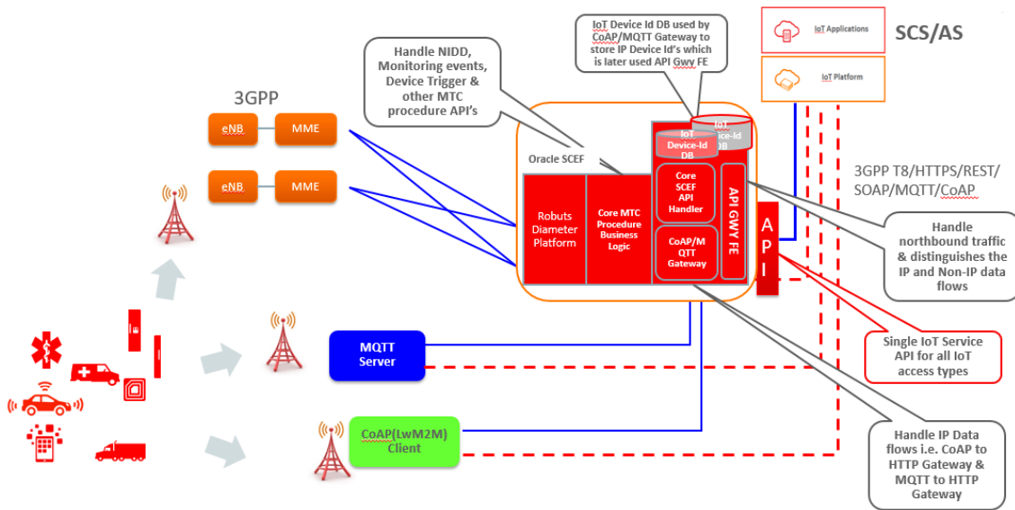
Figure 70: SCEF LWM2M Server, MQTT architecture example
