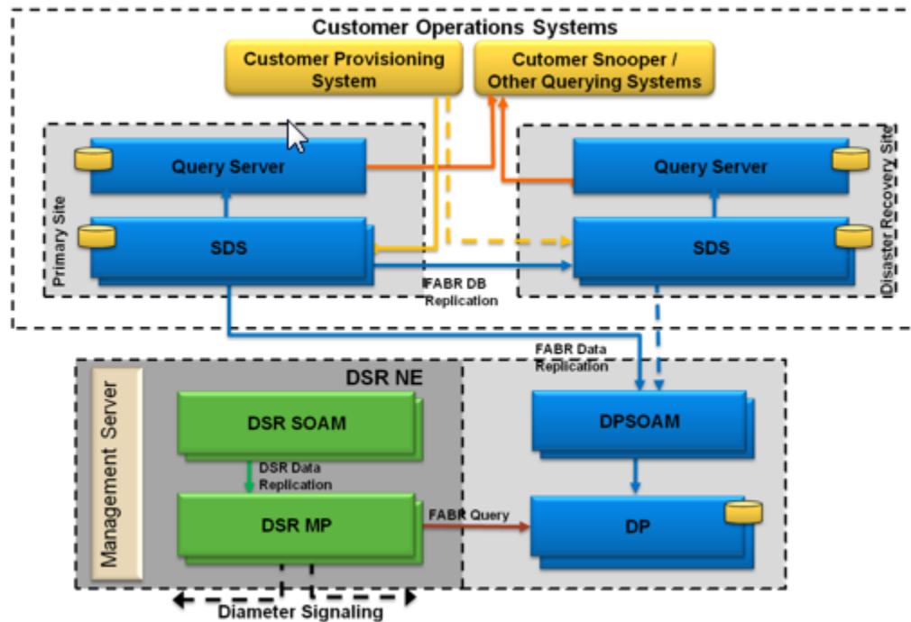
Figure 53 - Subscriber Data Server Architecture
