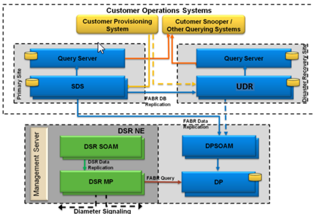
Figure 54 – User Data Repository Architecture
