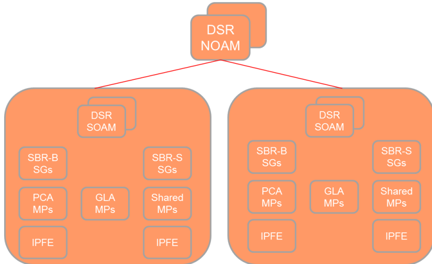
Figure 65 - PCA and GLA NOAM Architecture
