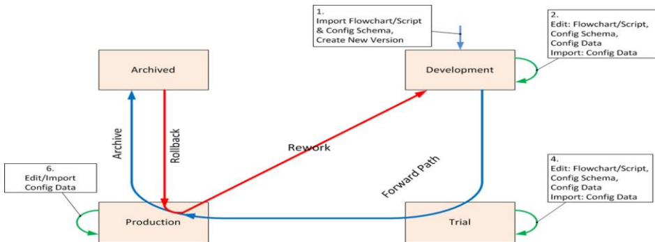
Figure 74 – Custom Application Framework (CAF) Application State Transitions
